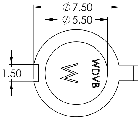
TOP VIEW PART NO. WD19 PART NO. WD39
