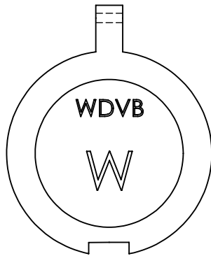
PLAN - PART NO. WD19 HINGE WIDTH 25mm (1")
