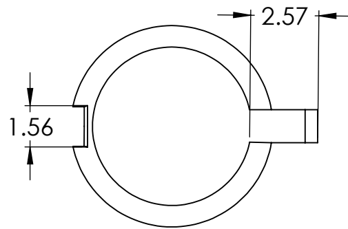
BOTTOM VIEW PART NO. WD19 PART NO. WD39
