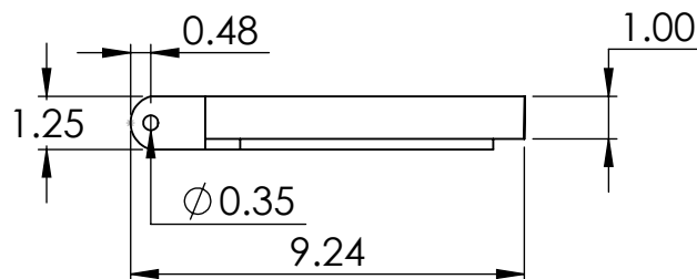
SIDE VIEW PART NO. WD19 PART NO. WD39
